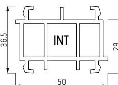
Podštok INT 6 m (Inoutic 70 Arkada, 76 Prestige) PMSLB.INT 9.80€
