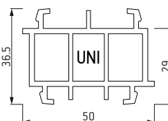
Podštok UNI 6 m (LB.Profile 82 mm, Salamander, Veka 70/80, Rehau 70/80/86, Profine 70, Gealan 8000/900) PMSLB.UNI 9.80€
