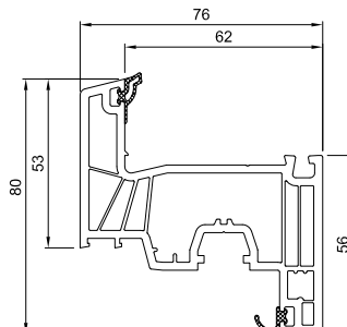
Krilo 76 mm MD - Antracit
